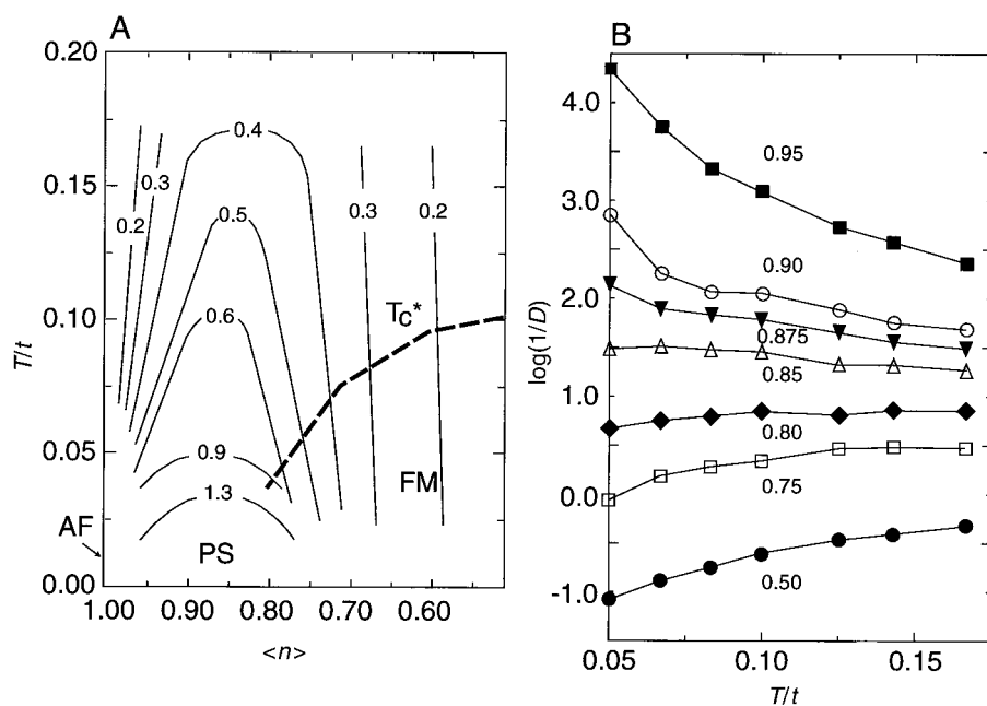
Fig. 3. (A) Lines of constant \kappa \langle n \rangle^2 = d\langle n \rangle / d\mu that correspond to the one-orbital model with J_H = \infty in the plane temperature \langle n \rangle ( e_g density). Plots were obtained from MC simulations with a 30-site chain with periodic boundary conditions. Coupling among the localized t_{2g} spins is J' = 0.05t and t is the hopping amplitude. T_C^* is a characteristic temperature where the zero-momentum Fourier-transform of the spin-spin correlations starts growing very rapidly as the temperature is reduced (9–11). (B) Plot of \log(1/D) versus T/t for the same model and cluster as in (A). D is the Drude weight obtained from the optical conductivity (11). Densities are indicated.
