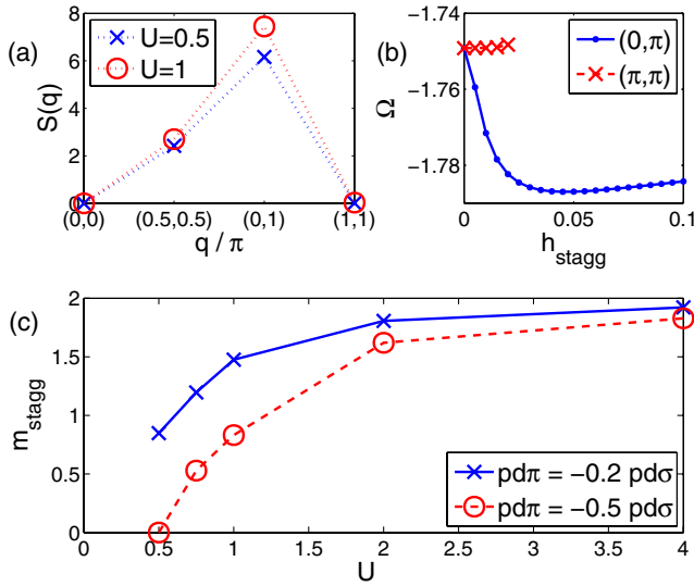
FIG. 2 (color online). (a) S(q) vs q for the \sqrt{8} \times \sqrt{8} cluster at the U 's indicated, with J = U/4 and pd\pi/pd\sigma = -0.2 . The momenta allowed in this cluster are (0, 0), (\pm \pi/2, \pm \pi/2), (0, \pi), (\pi, 0) , and (\pi, \pi) [30]. (b) VCA grand potential [in energy units (pd\sigma)^2/\Delta_{pd} ] vs staggered magnetic fields h_{\text{stagg}} for q = (\pi, \pi) and (0, \pi) , and pd\pi/pd\sigma = -0.2 , U = 1 , J = 0.25 . The minimum for (0, \pi) at h_{\text{stagg}} \neq 0 indicates symmetry breaking. (c) m_{\text{stagg}} vs U , with U/J = 4 . The small U region at pd\pi/pd\sigma = -0.2 was numerically unstable.
